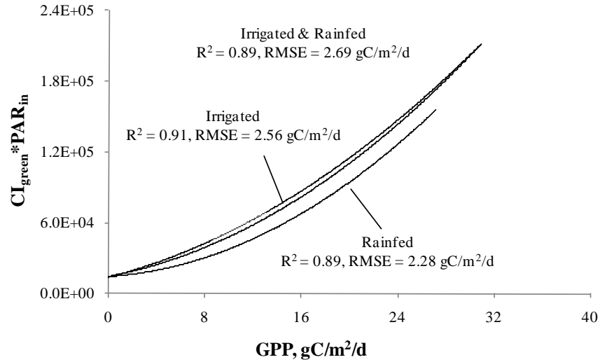
Fig. 5. Best fit functions of the relationships between daily gross primary production and the products of CI_{\text{green}} \times \text{PAR} . Dotted line: 12 irrigated sites in 2001 through 2008, dashed line: 4 rainfed sites in 2002, 2004, 2006, and 2008, solid line: 16 irrigated and rainfed sites taken together.
