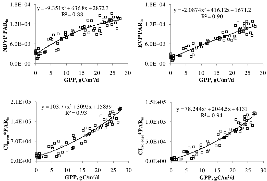
Fig. 2. Relationships between daytime gross primary production in irrigated sites in 2003 and the product of vegetation index and incident PAR for four vegetation indices: NDVI, EVI2, CI_{green} , and CI_{red\ edge} .
