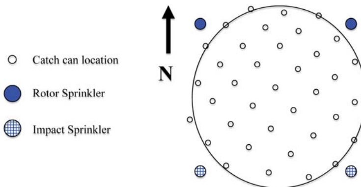
Figure 1. Layout of sprinklers and catch cans on Hole 18.
