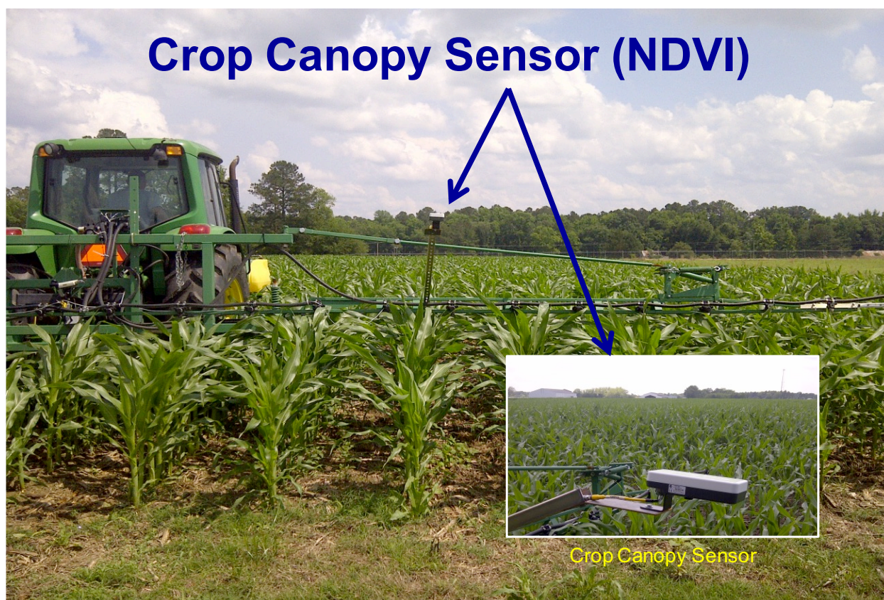
Figure 1. NDVI crop canopy sensor mounted on tractor spray boom.
