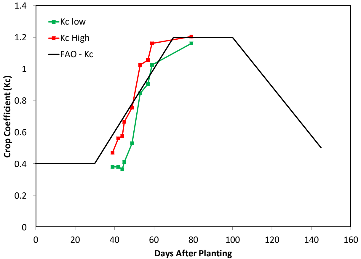
Figure 4. NDVI based crop coefficients for cotton.
