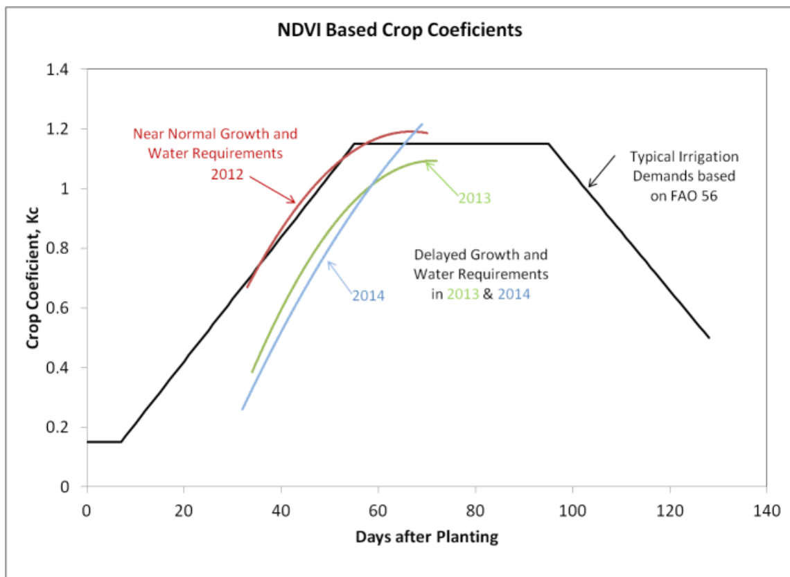
Figure 3. NDVI based crop coefficients for the 2012-2014 corn crops.
